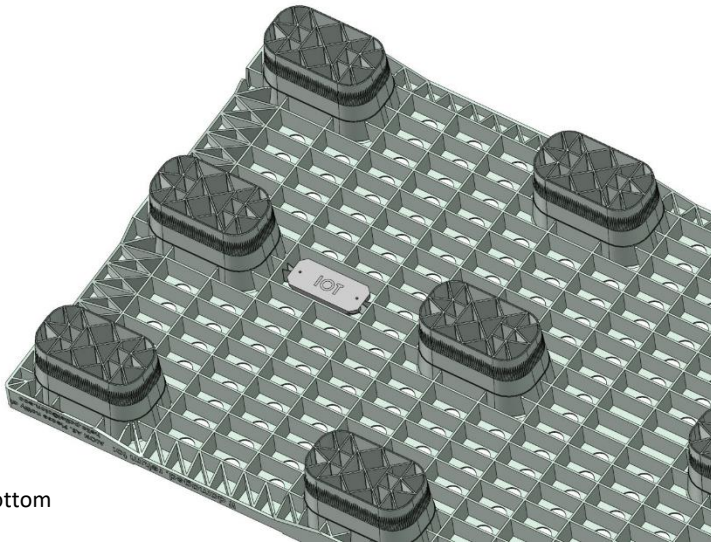
Fig. 2 – AION Nestable pallet stacked on a full truck (1485 pallets)
