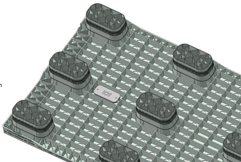
Fig. 4 – AION Nestable pallet design bottom
