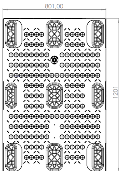
Fig. 1 – AION Nestable pallet design w/ dimensions (mm)
